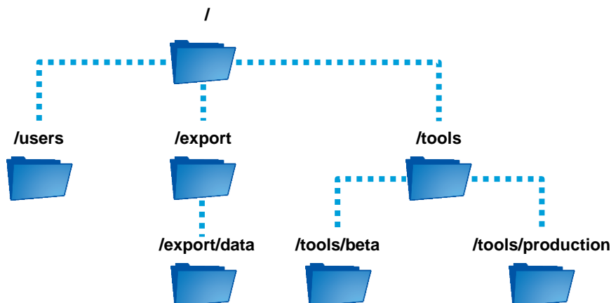
Figure 3) A nested SVM namespace. A dotted line represents a junction. The volumes located in /export/data , /tools/beta , and /tools/production are junctioned off data volumes, not the SVM root volume.
