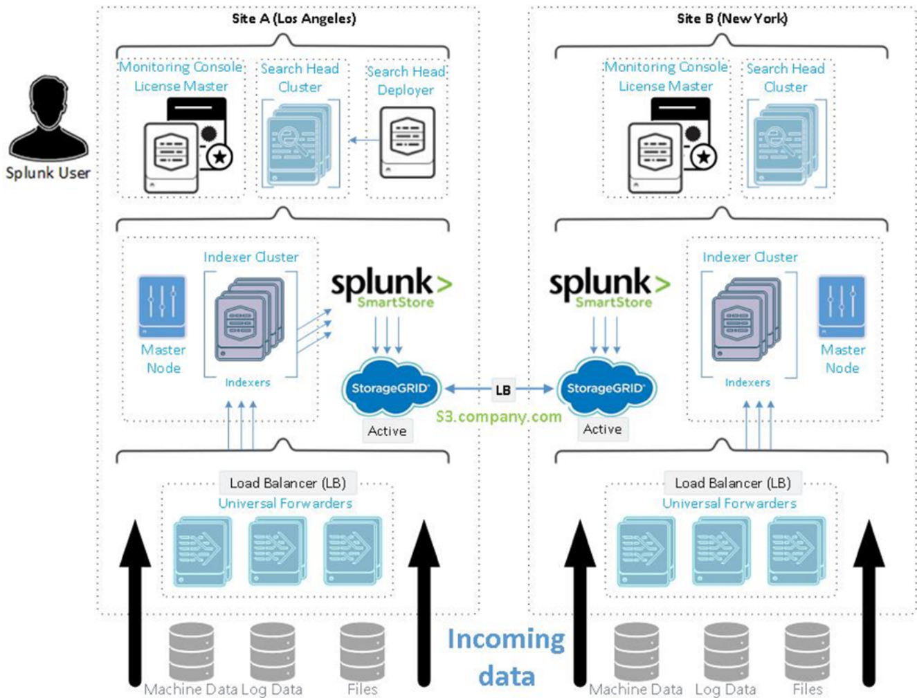
Figure 1) Splunk SmartStore multisite deployment with NetApp StorageGRID.
