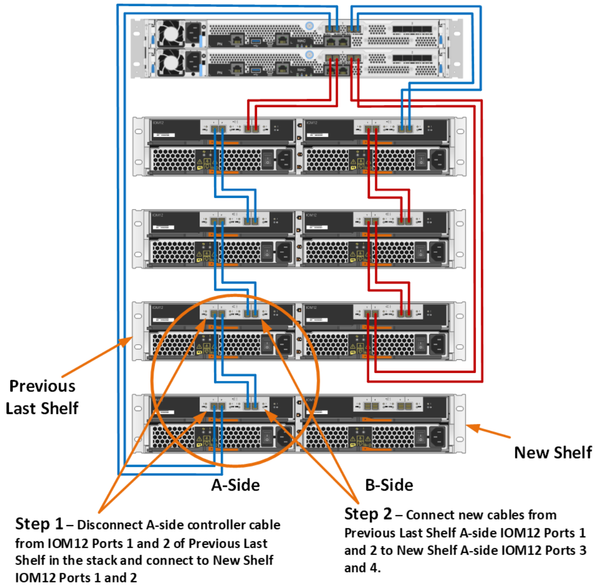
Figure 49) Drive shelf hot-add A-side cabling.
