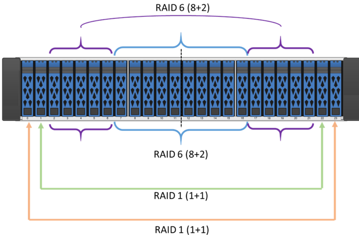
Figure 8) Example of using all 24 drives in a configuration.
