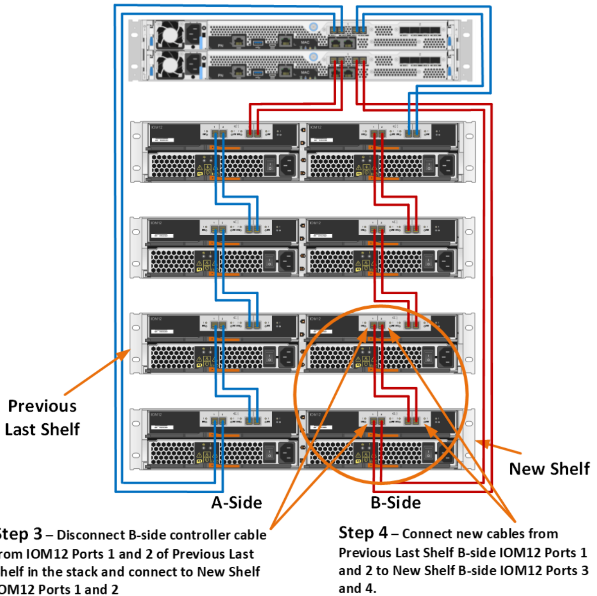
Figure 50) Drive shelf hot-add B-side cabling.
