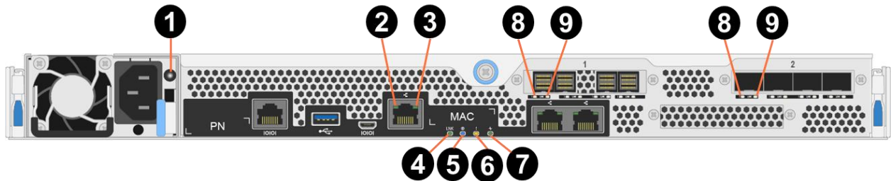
Figure 44) LEDs on the EF300 (4-port HIC and SAS expander shown).
