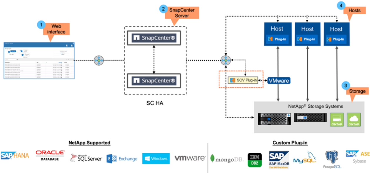
Figure 1) SnapCenter supports a variety of applications and protocols. Consult the NetApp Interoperability Matrix Tool (IMT) for details.
