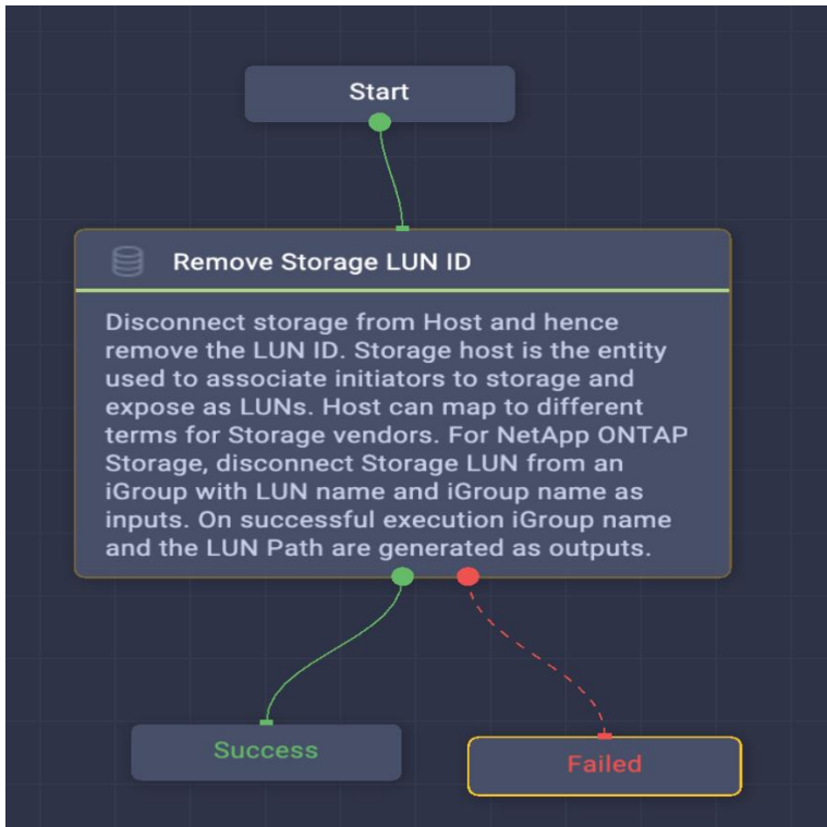
Figure 29) Task #19: Remove storage LUN ID.
