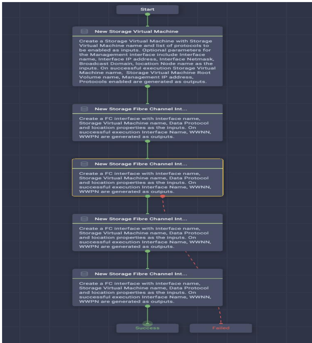
Figure 45) Custom-defined workflow #1.
