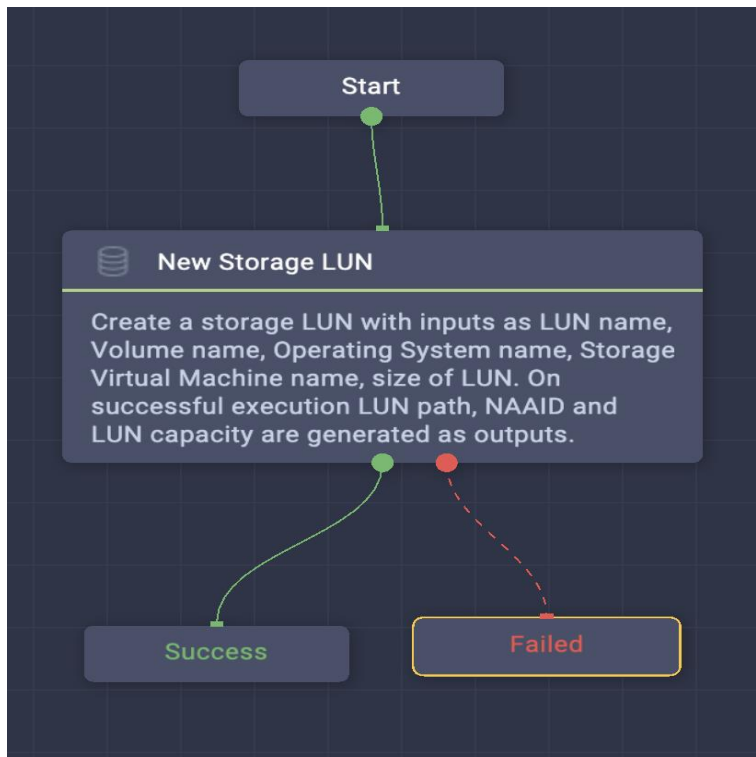
Figure 22) Task #12: New storage LUN.
