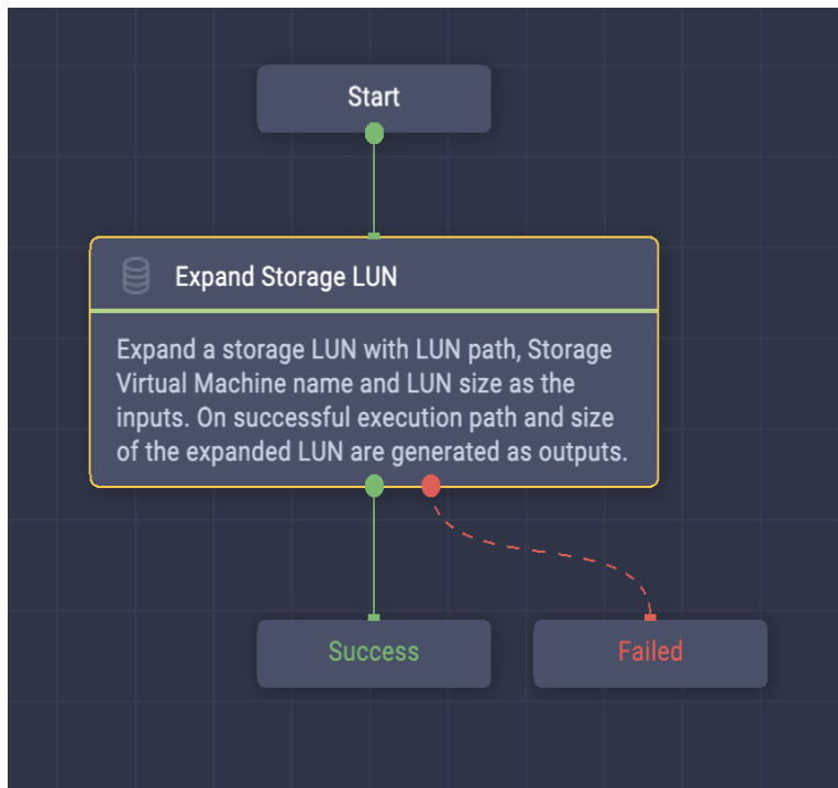
Figure 13) Task #3: Expand Storage LUN.
