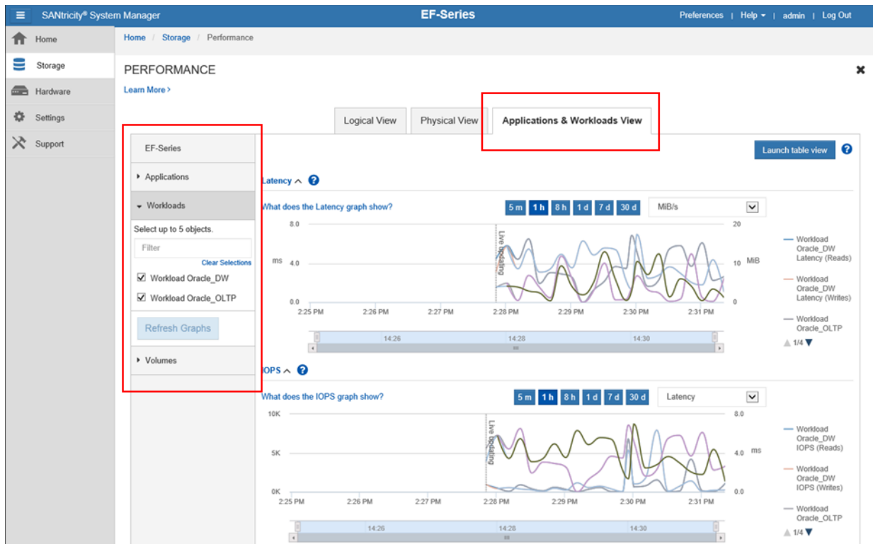
Figure 9) Example of Performance Monitor with Applications & Workloads View.
