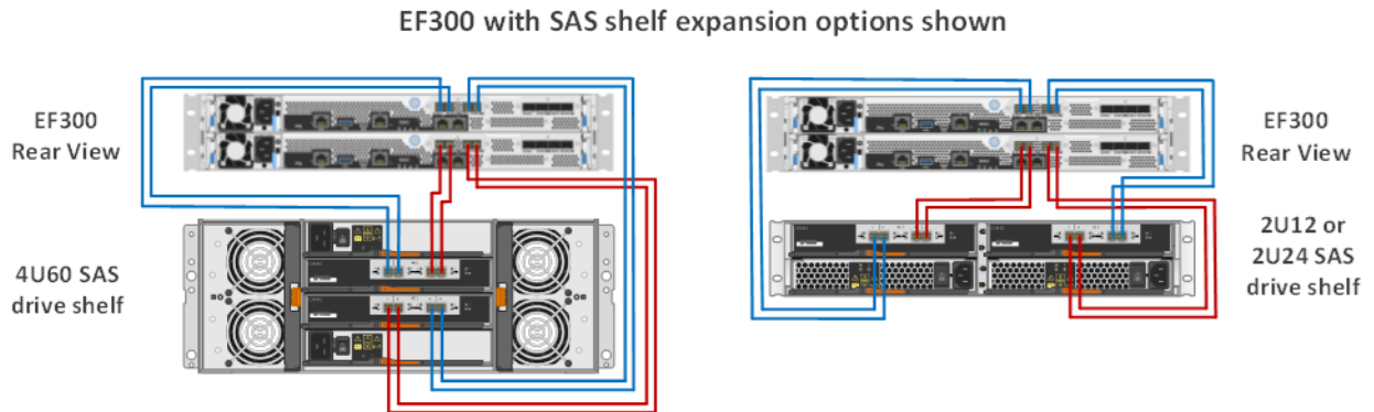
Figure 1) EF300 with SAS expansion configuration.
