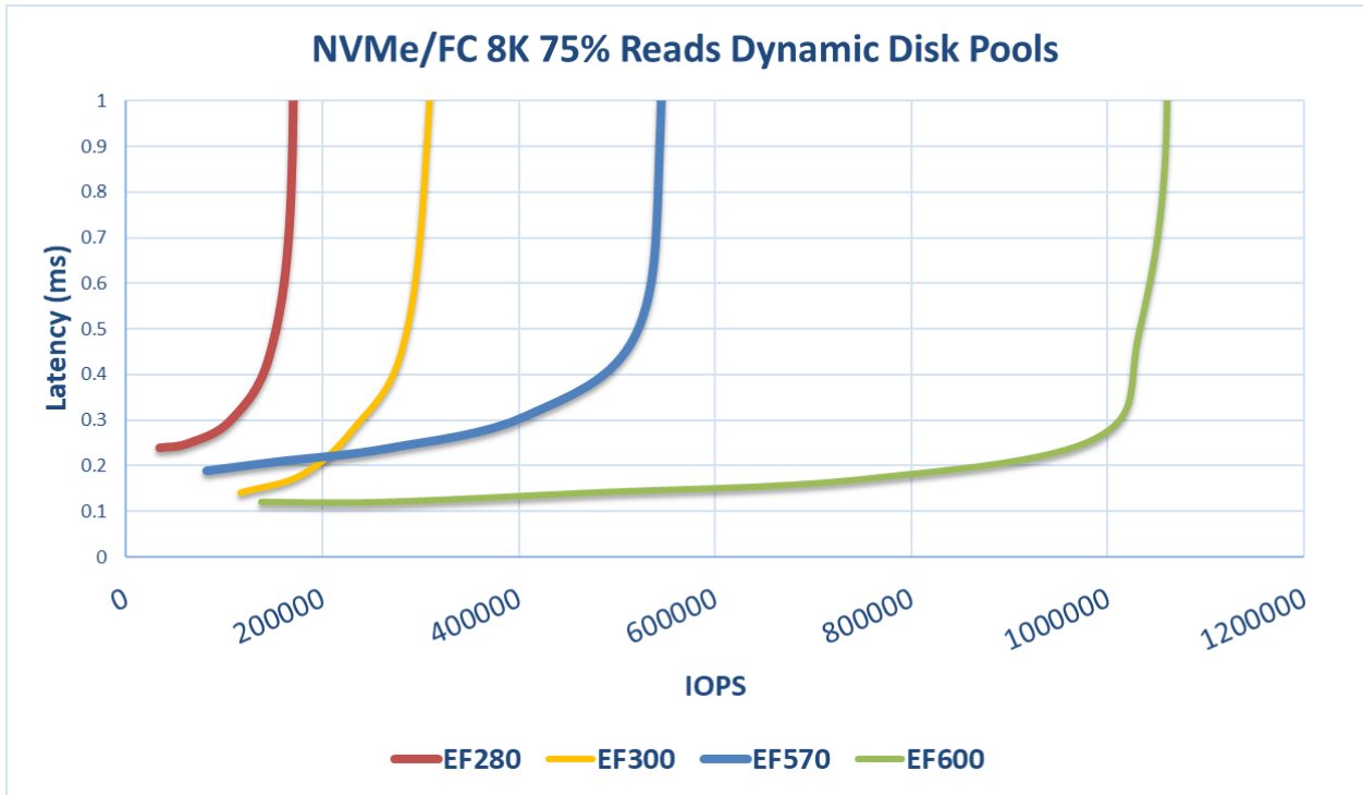
Figure 5) Performance results comparison for OLTP configuration.
