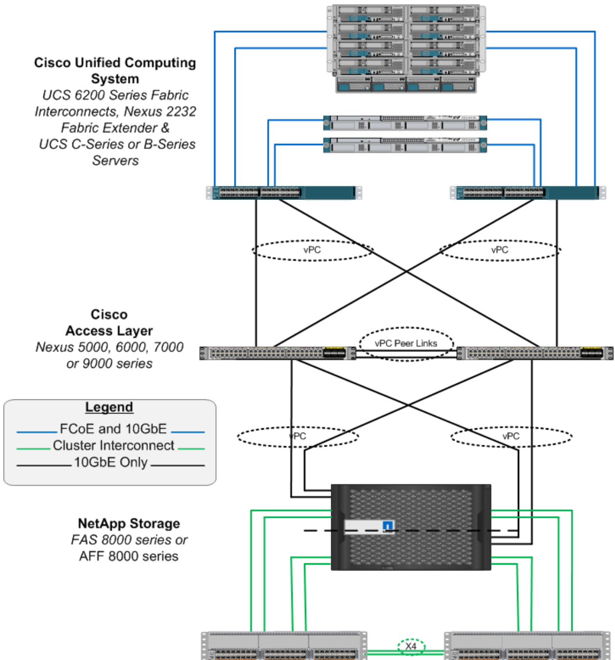
Figure 6) iSCSI boot FlexPod infrastructure.
