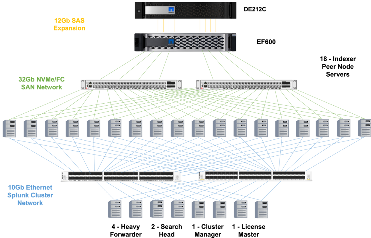
Figure 3) Splunk cluster with E-Series.
