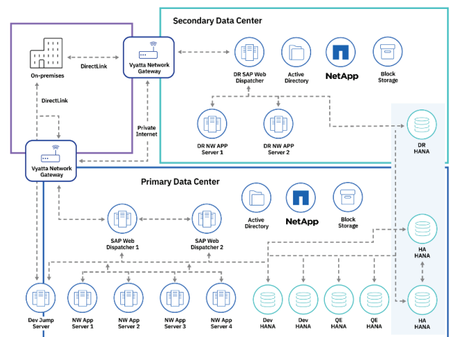
Figure 1: Reference architecture.
