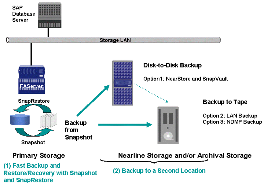
Figure 16) SAP backup and recovery—NetApp solution overview.
