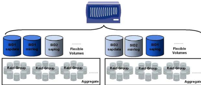
Figure 3) Storage layout with three FlexVol volumes.
