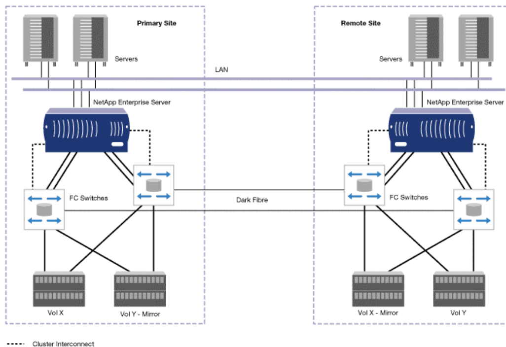
Figure 20) MetroCluster over direct Fibre Channel switch connection.
