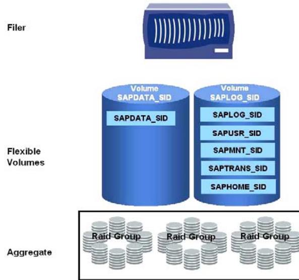
Figure 10) Installation with three FlexVol volumes.
