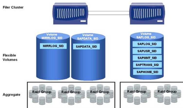
Figure 9) Installation with three FlexVol volumes in a storage system cluster.
