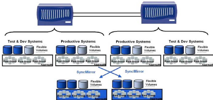
Figure 6) Storage layout with NetApp MetroCluster and aggregates.
