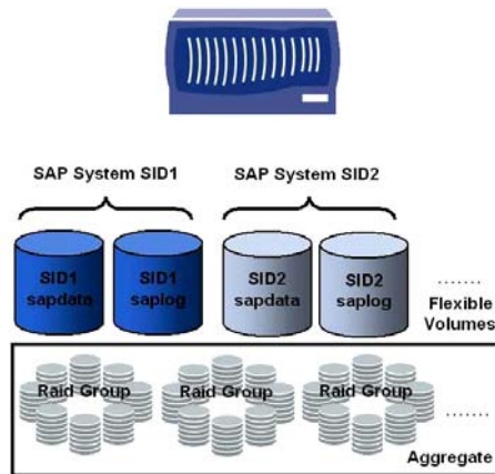
Figure 4) Storage layout with two FlexVol volumes.
