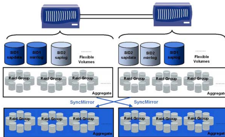
Figure 5) Storage layout with NetApp MetroCluster.
