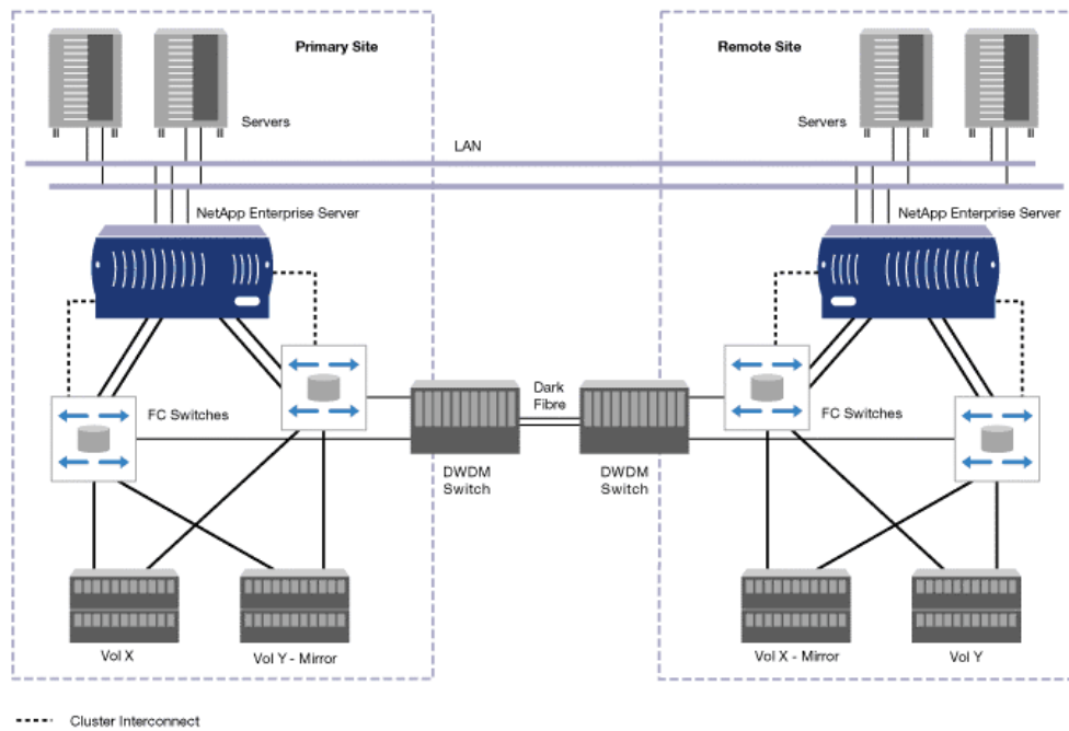
Figure 21) MetroCluster over Fibre Channel and DWDM switch infrastructure.
