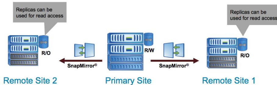
Figure 2) Remote read access to SnapMirror replicas.
