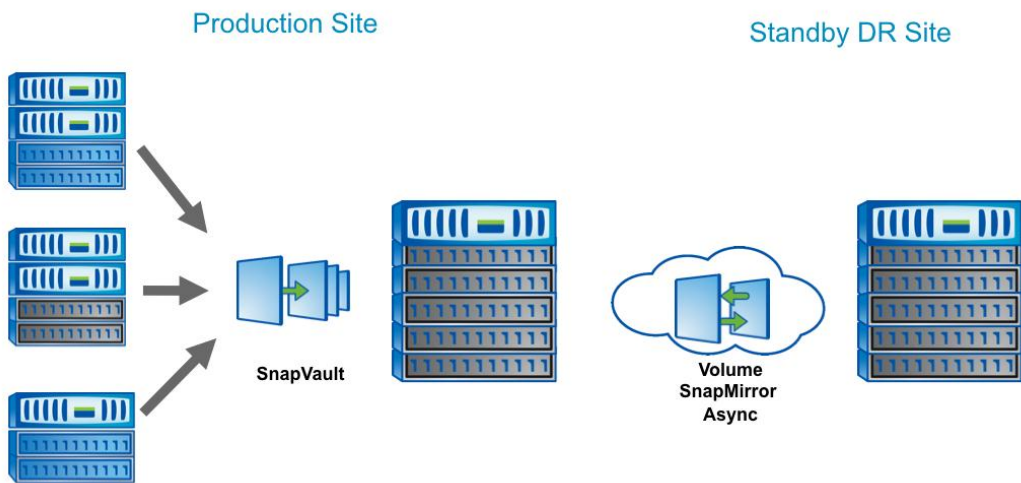
Figure 18) Example of DR protection for backup data.
