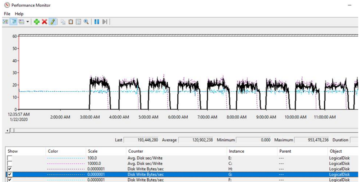
Figure 19) Scenario 2: E2812 tier 1, E5760 tier 2 400-camera throughput during archiving.
