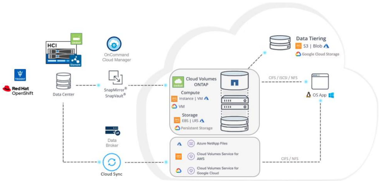
Figure 1) Solution architecture.
