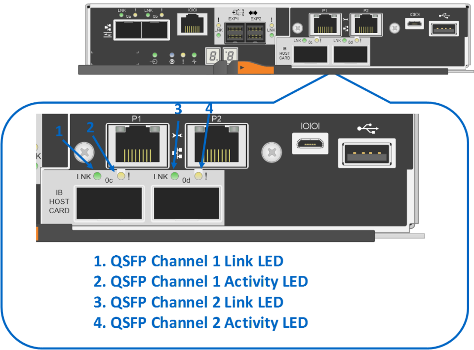
Figure 44) LEDs on 2-port 100Gb IB HIC.
