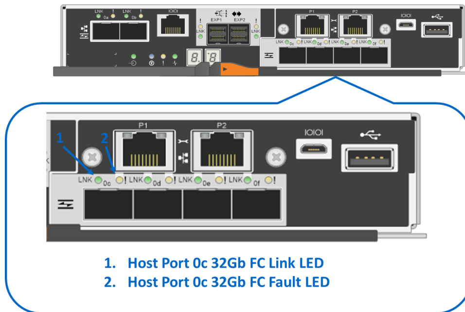
Figure 46) LEDs for 4-port 32Gb FC HIC.
