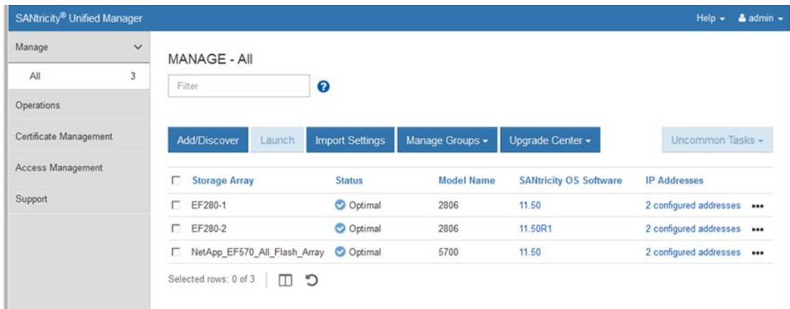
Figure 10) SANtricity Unified Manager landing page.
