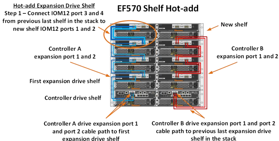
Figure 56) Drive shelf hot-add controller expansion port 1 cabling.
