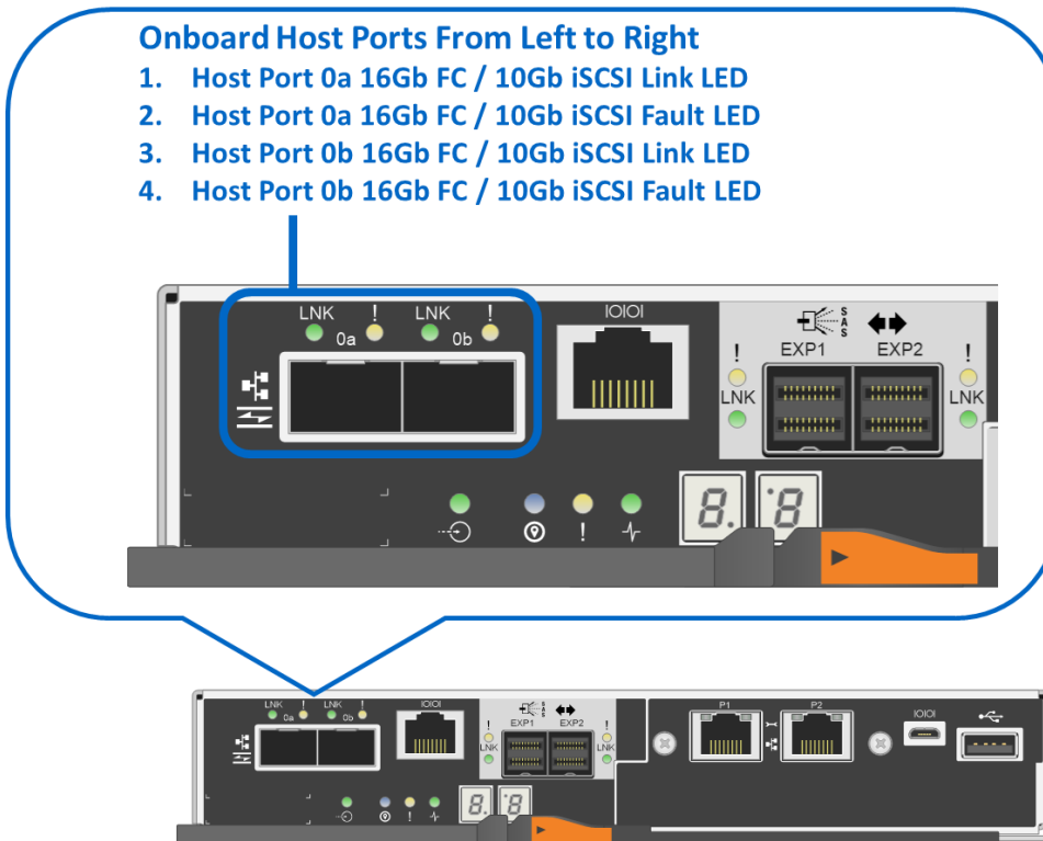
Figure 42) Ports 0a and 0b 16Gb FC/10Gb iSCSI baseboard host ports.
