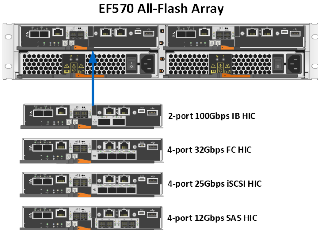
Figure 35) EF570 with optional HICs.
