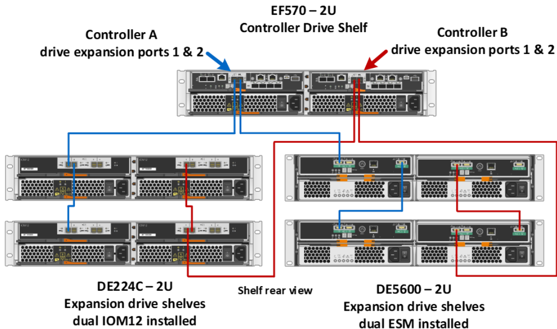
Figure 55) EF570 with mixed 6Gbps and 12Gbps expansion shelves.
