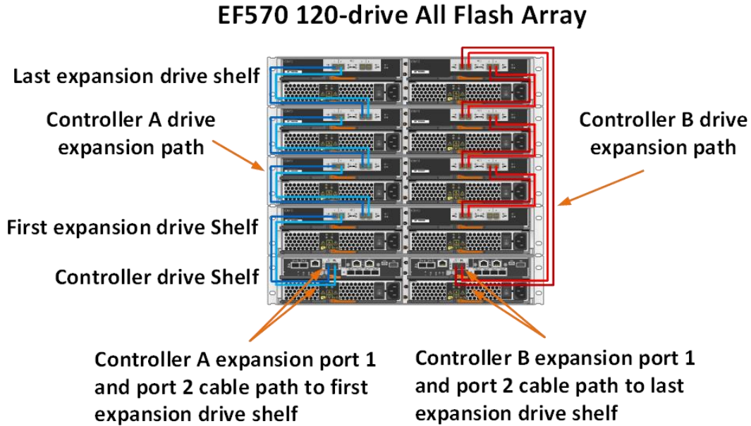
Figure 54) EF570 expansion-drive shelf cabling example for maximum DE224C shelf configuration.
