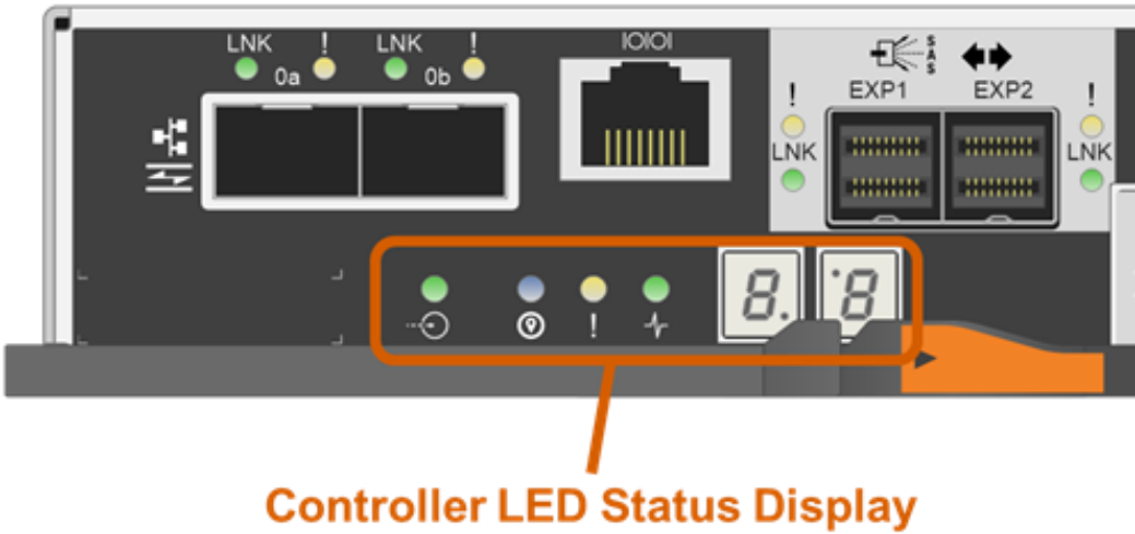
Figure 40) Controller module and array status LEDs.
