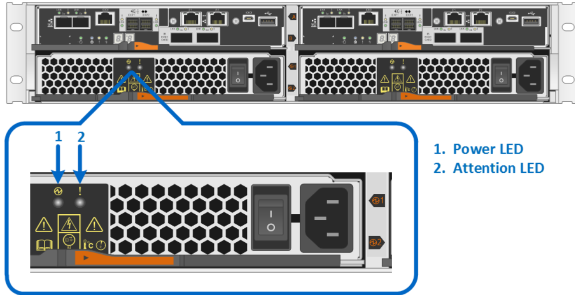
Figure 38) LEDs on EF570 power fan canister (rear view).
