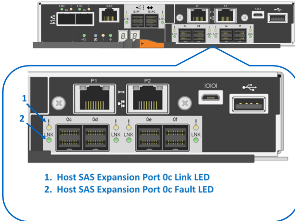
Figure 45) LEDs for 4-port 12Gb SAS HIC.
