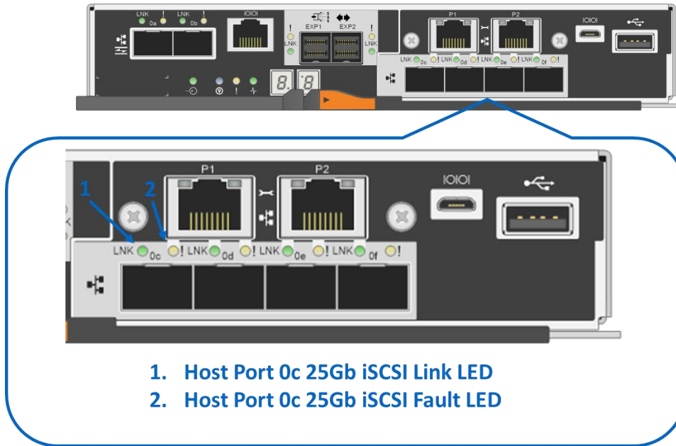
Figure 47) LEDs for 4-port 25Gb iSCSI HIC.
