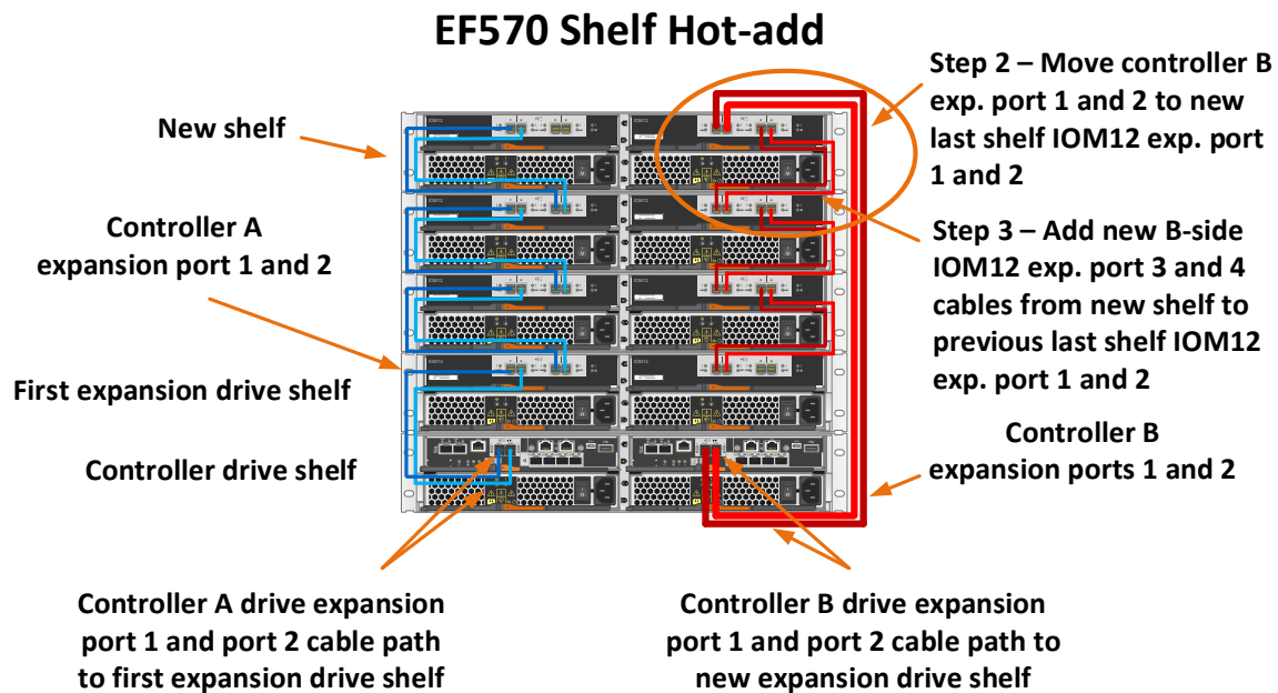
Figure 57) Drive shelf hot-add controller expansion port 2 cabling.
