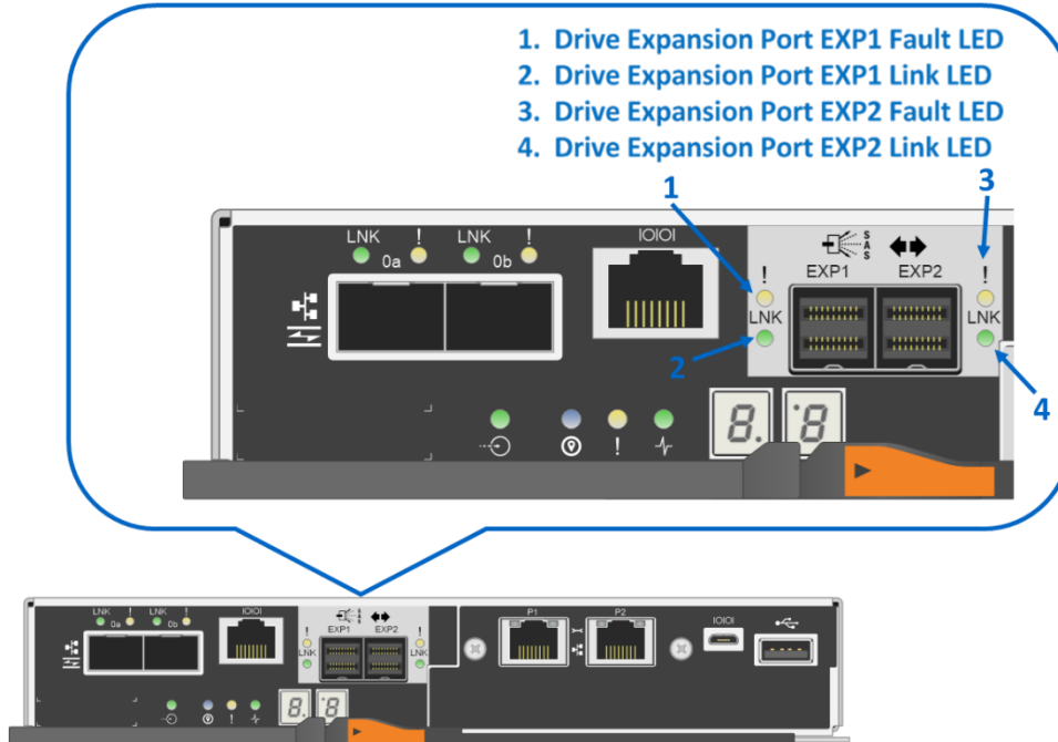
Figure 43) LEDs for drive expansion ports.
