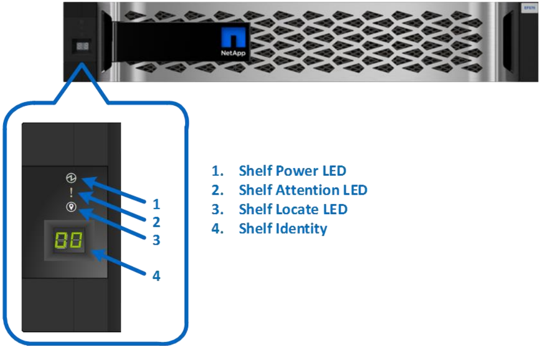
Figure 36) ODP on front panel of EF570 controller shelf.
