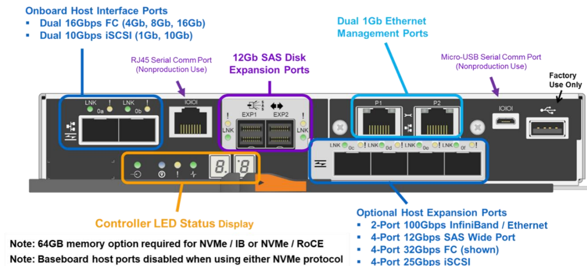
Figure 2) EF570 controller with ports identified.
