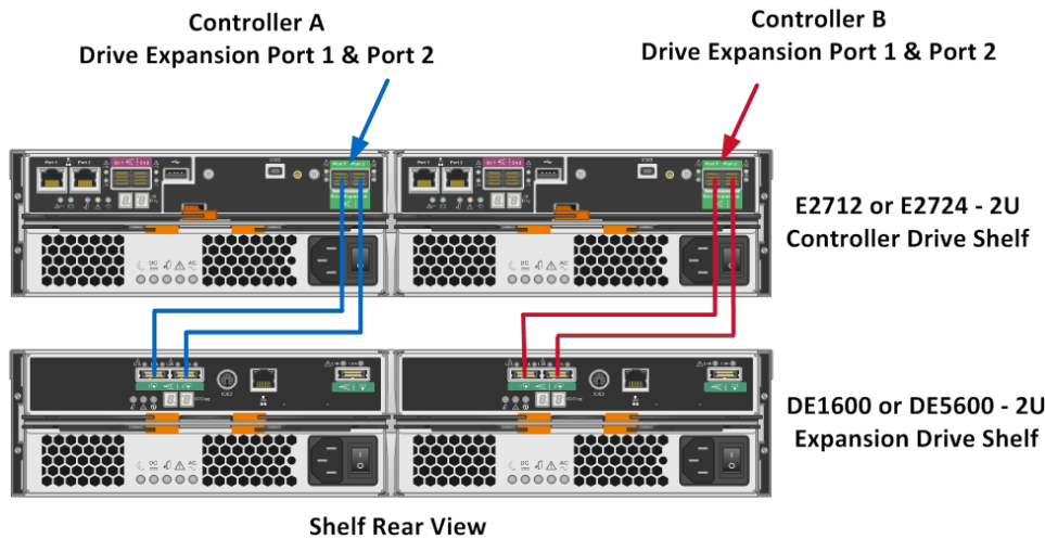
Figure 26) E2700 single-stack system configuration.
