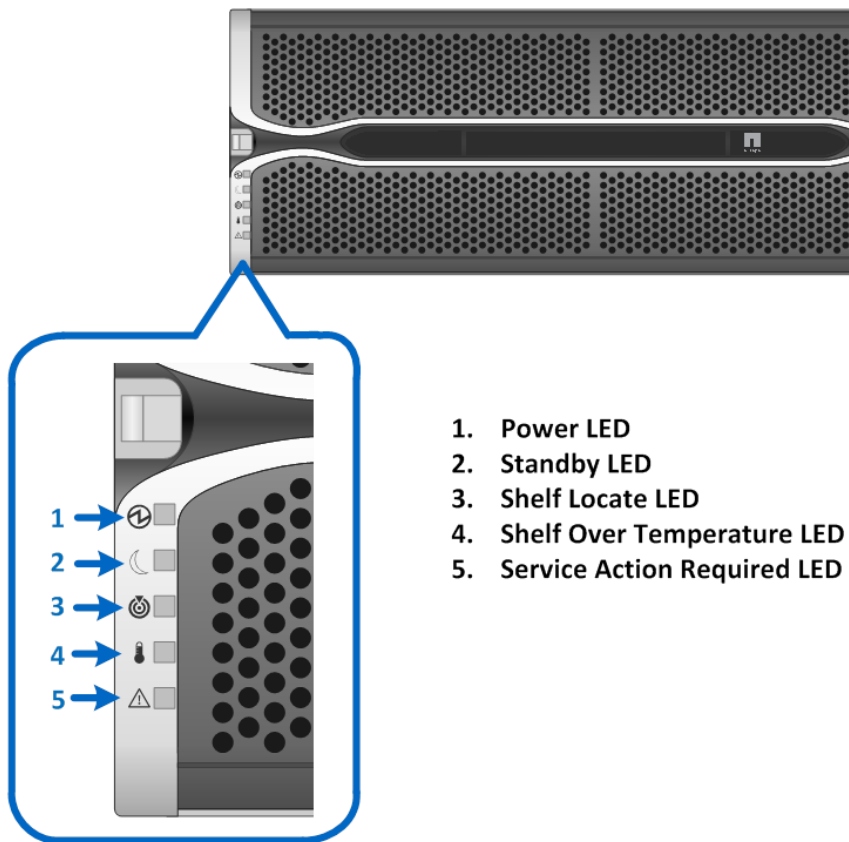
Figure 14) LEDs on front panel of E2760 controller-drive shelf.
