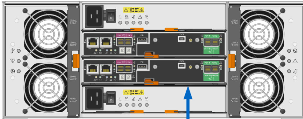
E2760 4U Tray Rear View with Dual E2700 Controllers
