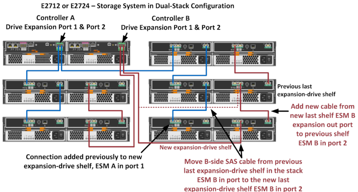
Figure 30) Drive shelf hot-add B-side cabling.
