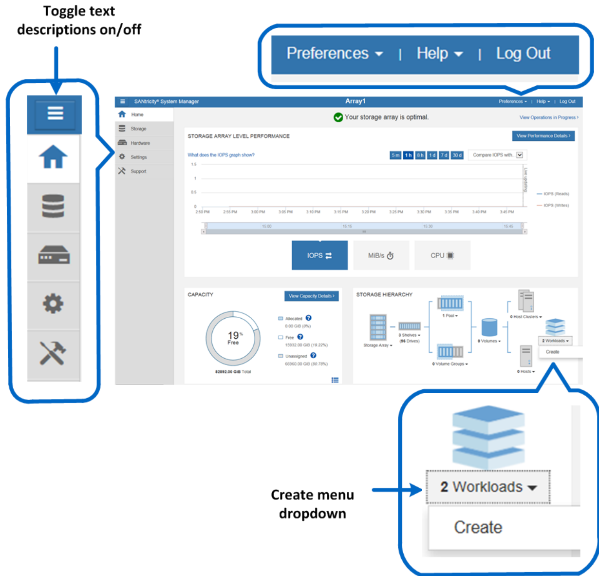
Figure 14) System Manager home page.
