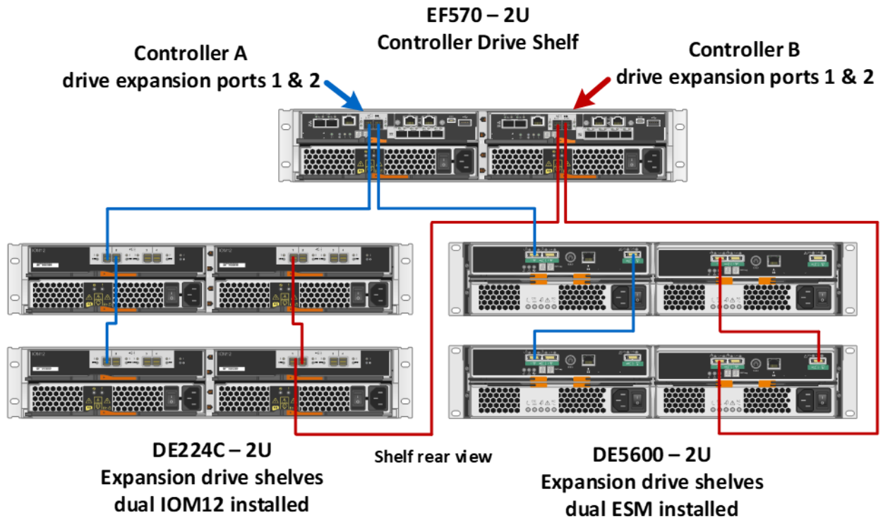
Figure 48) EF570 with mixed 6Gbps and 12Gbps expansion shelves.
