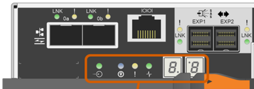
Figure 33) Controller module and array status LEDs.
