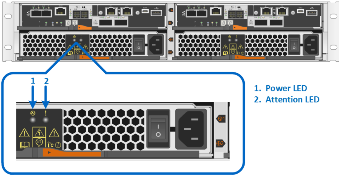
Figure 31) LEDs on EF570 power-fan canister (rear view).
