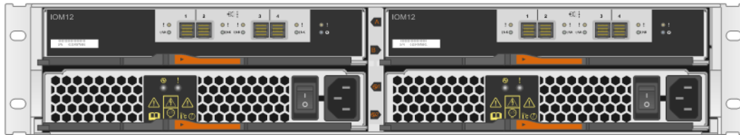
Figure 44) DE224C rear view.
