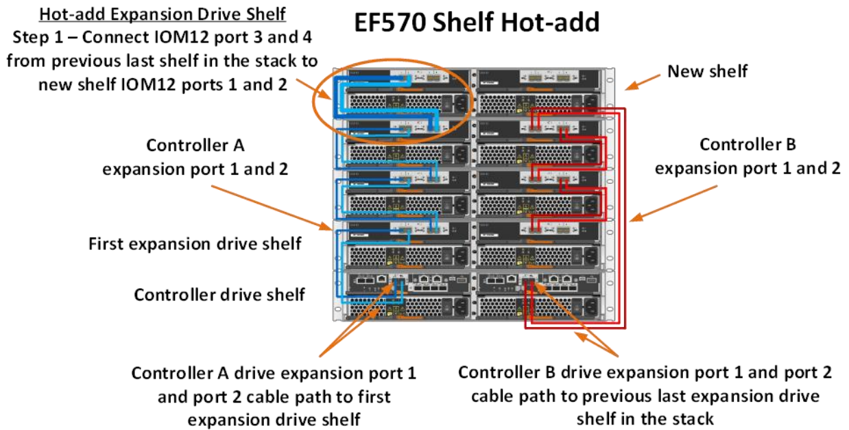
Figure 49) Drive shelf hot-add controller expansion port 1 cabling.
