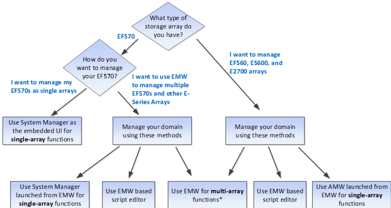
Figure 10) Decision tree for SANtricity management components to install.
