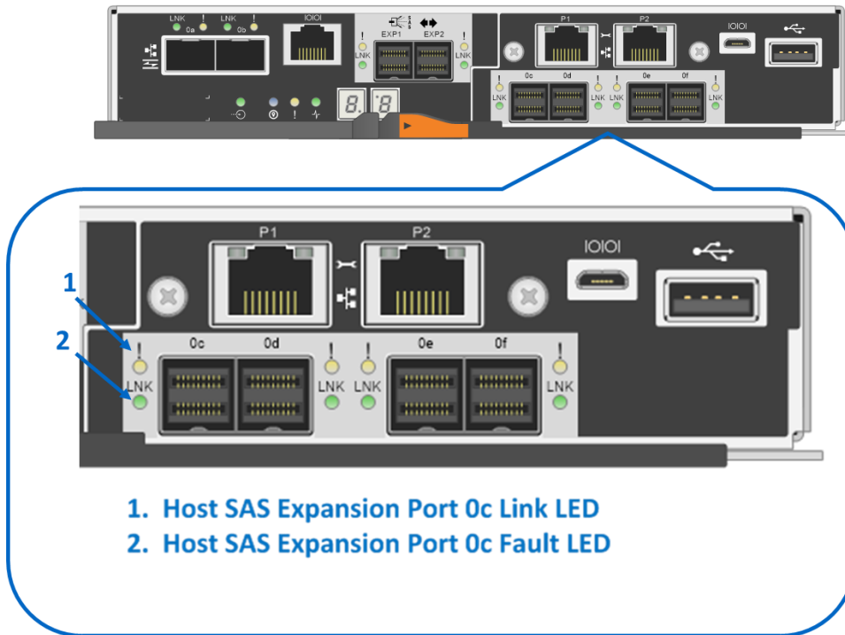
Figure 38) LEDs for 4-port 12Gb SAS HIC.
