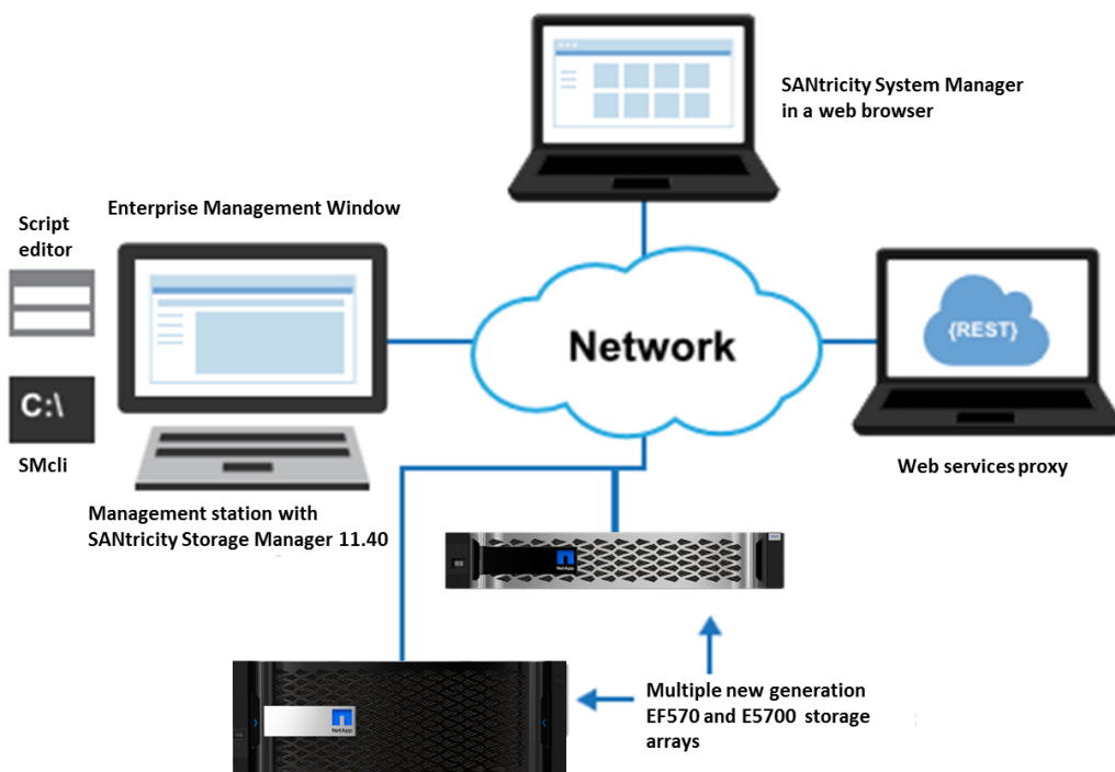
Figure 12) Managing multiple EF570 systems and E5700 systems with SANtricity Storage Manager and System Manager.
