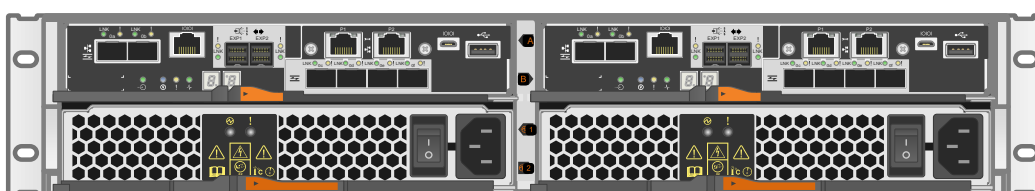
Figure 27) EF570 rear view.
