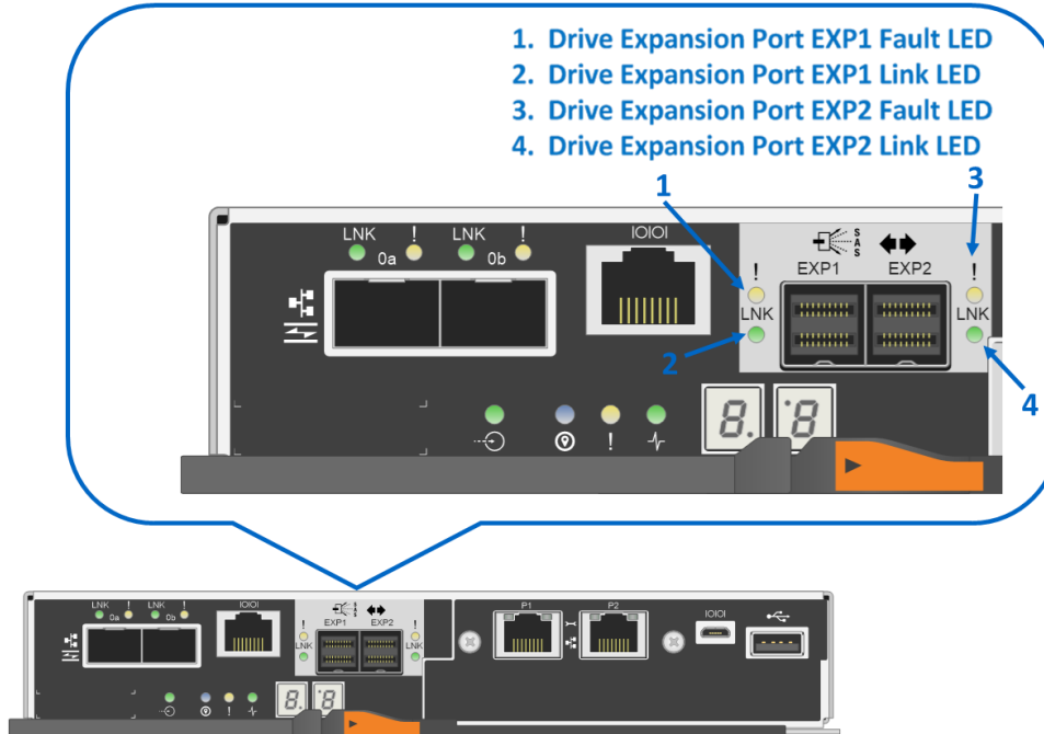
Figure 36) LEDs for drive expansion ports.
