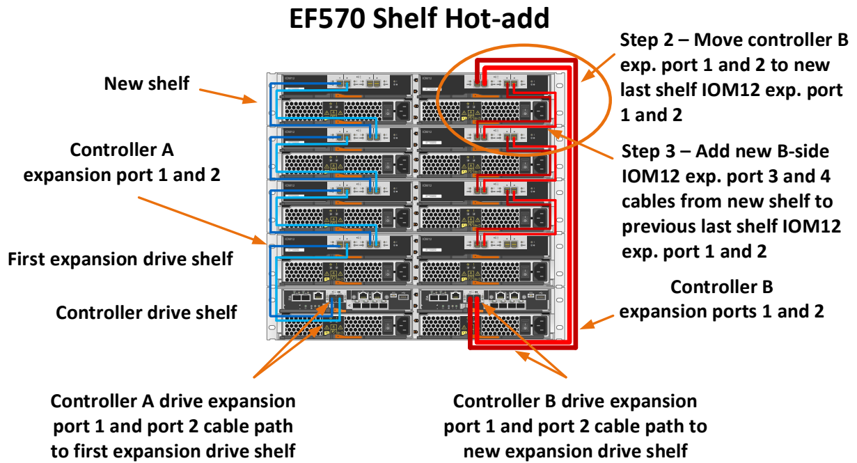
Figure 50) Drive shelf hot-add controller expansion port 2 cabling.
