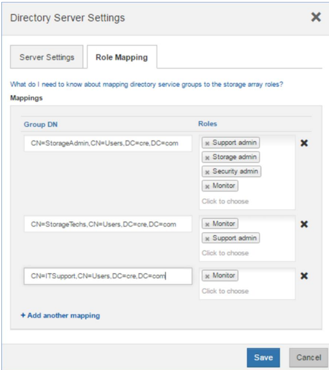
Figure 5) Role Mapping tab in the Directory Server Settings wizard.
