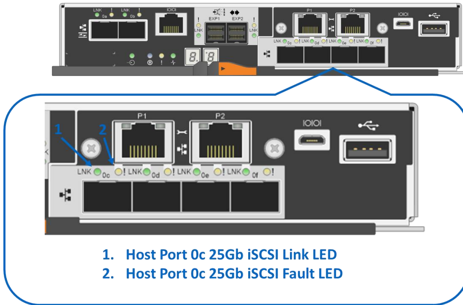
Figure 40) LEDs for 4-port 25Gb iSCSI HIC.
