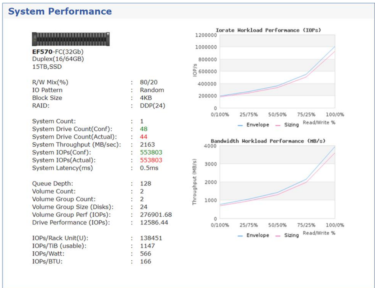
Figure 24) Performance sizing report.
