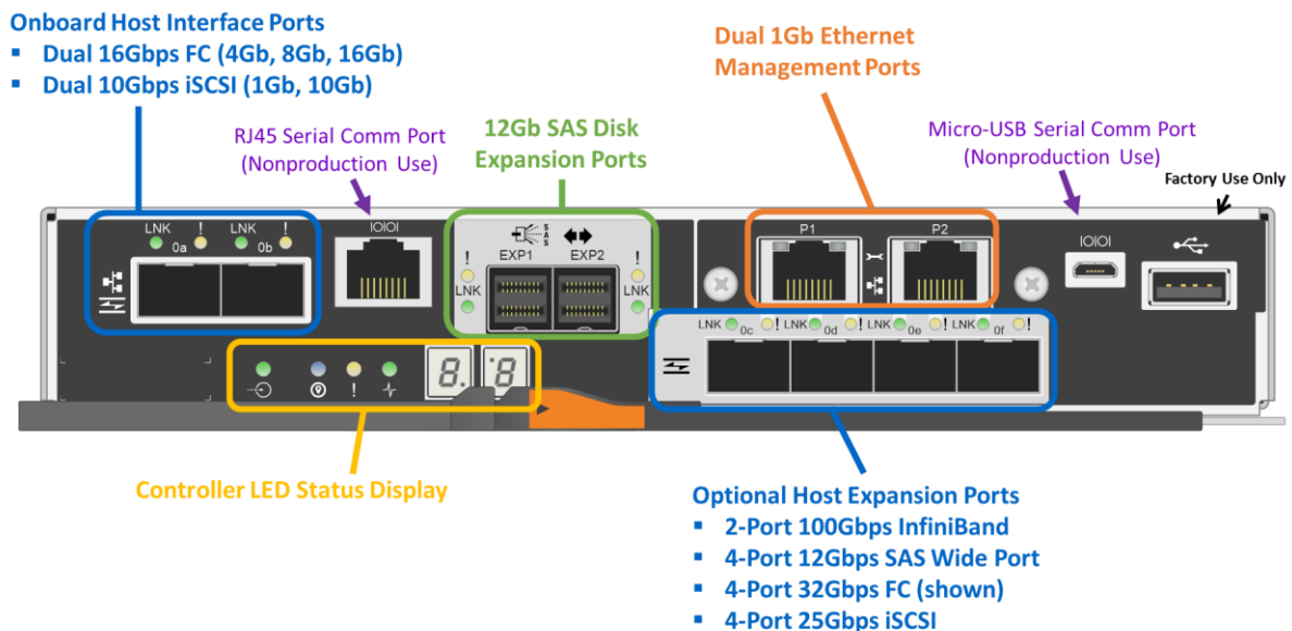
Figure 3) EF570 controller with ports identified.
