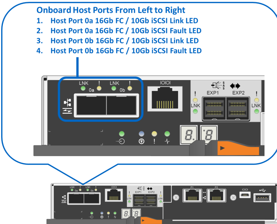
Figure 35) Ports 0a and 0b 16Gb FC/10Gb iSCSI baseboard host ports.
