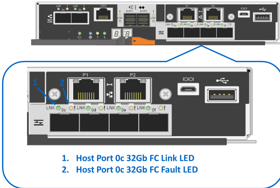
Figure 39) LEDs for 4-port 32Gb FC HIC.
