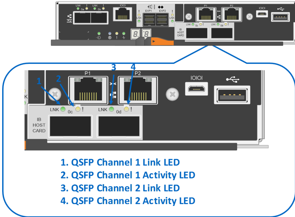
Figure 37) LEDs on 2-port 100Gb IB HIC.
