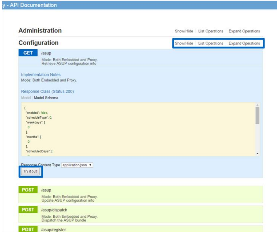
Figure 21) REST API documentation sample.
