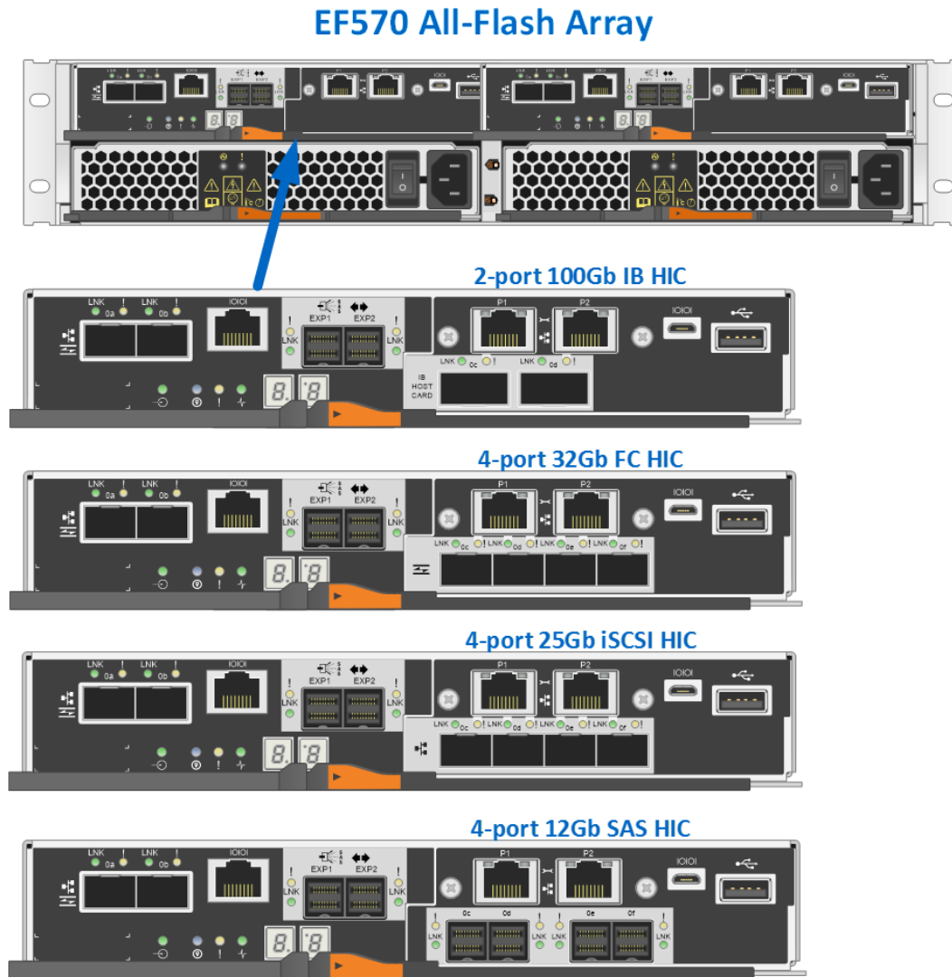
Figure 28) EF570 with optional HICs.
