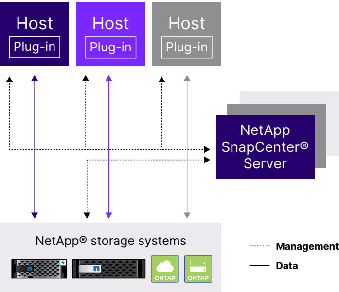
Figure 3: SnapCenter centralizes and simplifies data protection and clone management.
