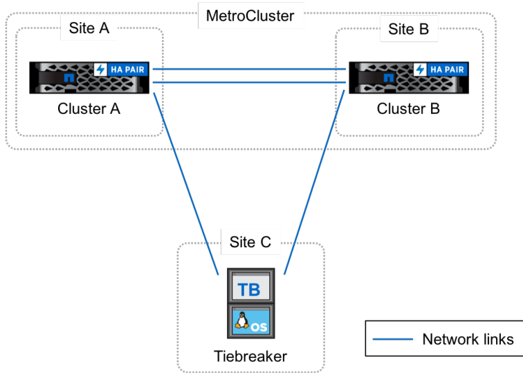
Figure 15) MetroCluster Tiebreaker site.
