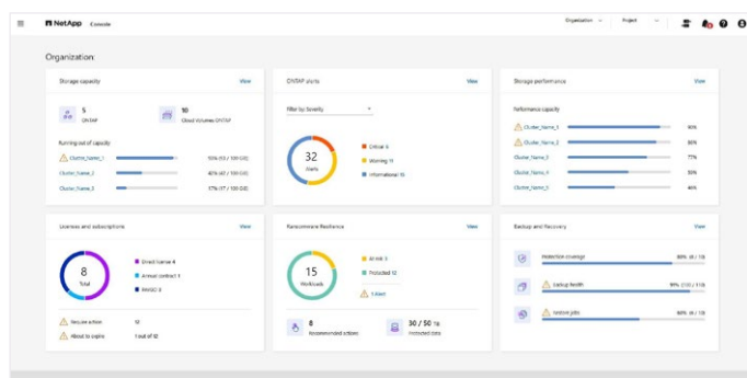
Figure 1 : NetApp Console
